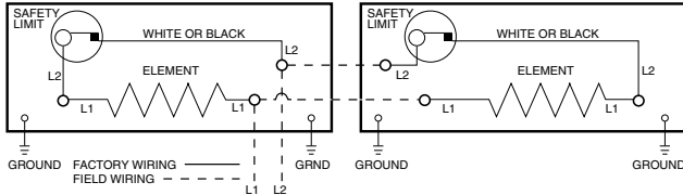
Figure 5: Wiring Diagrams
