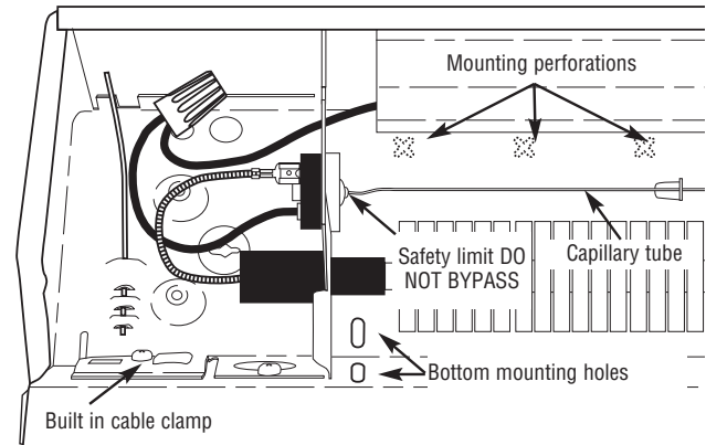
Figure 4: Left Side Wiring Compartment Shown
